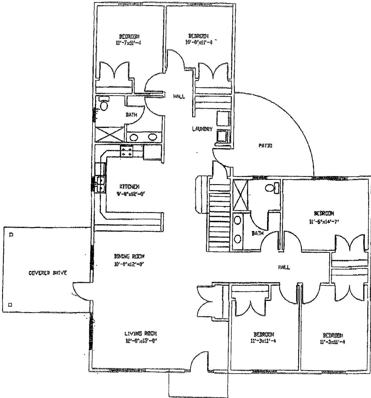
MAIN FLOOR PLAN SCALE: 1/8" = 1'-0" 2192 SF
