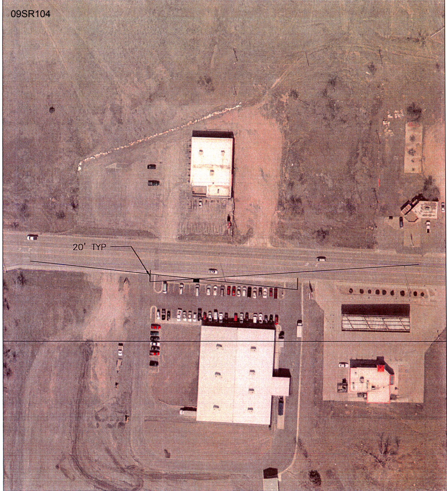
SALVATION ARMY TRANSIT SHELTER SIGHT TRIANGLE
