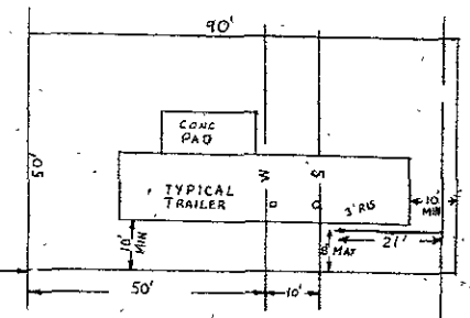
TYPICAL TRAILER LOT DETAIL SCALE 1" = 20'
