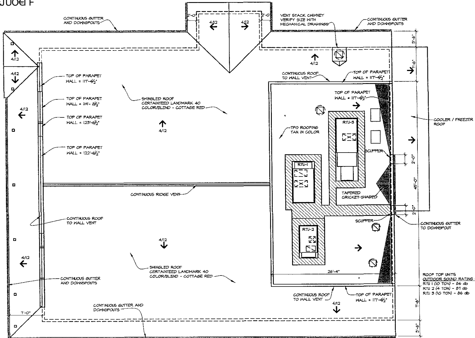
1 PROPOSED RESTAURANT ROOF PLAN A1.1 1/8" = 1'-0" NORTH
