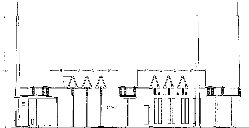
CLEVELAND STREET ELEVATION
