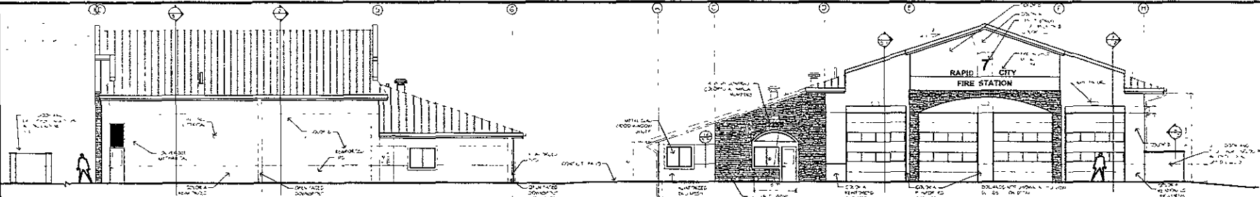
10 - 1.1 SIDE ELEVATION (NORTH) - ALTERNATE #2
