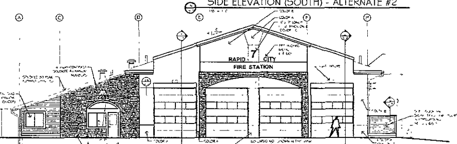
10 - 1.6 FRONT ELEVATION (EAST) - BASE BID
