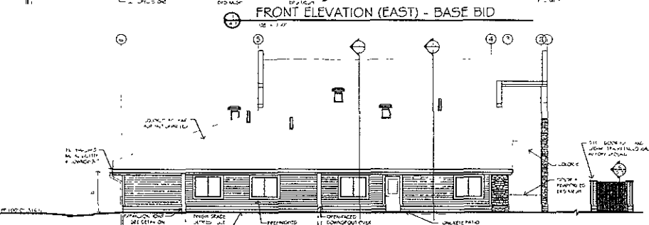
10 - 1.8 SIDE ELEVATION (SOUTH) - BASE BID
