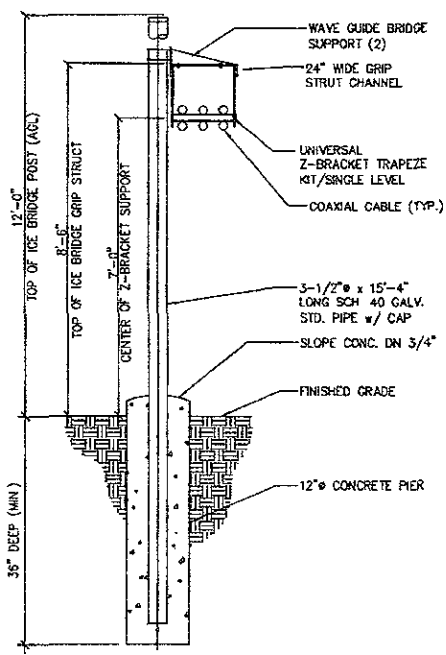
2 ICE BRIDGE DETAIL SCALE: NONE
