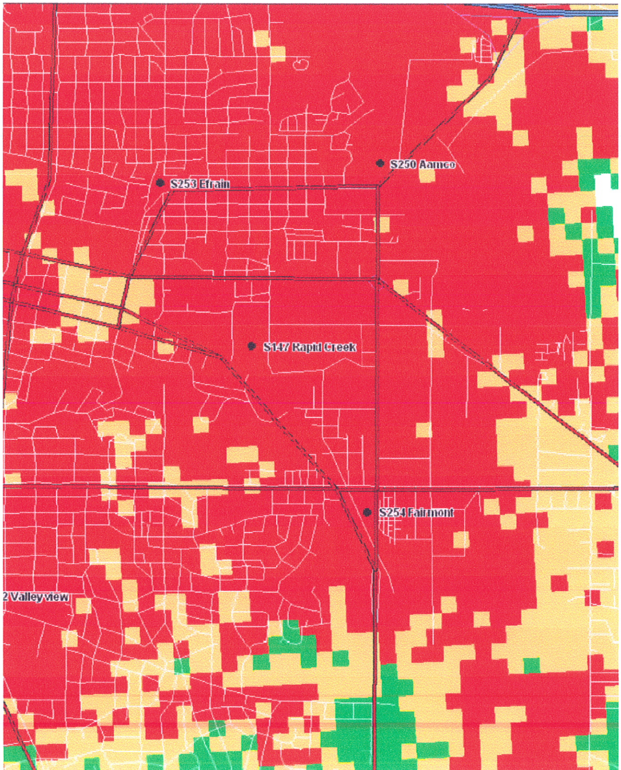
PROPAGATION (COVERAGE) MAP
