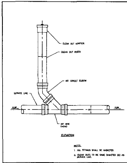
CITY OF RAPID CITY PUBLIC WORKS DEPARTMENT SANITARY SEWER SERVICE CLEAN OUT DETAIL DATE 5-1-07 SEC SHT 9-10
