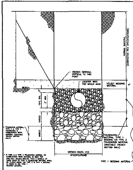
CITY OF RAPID CITY PUBLIC WORKS DEPARTMENT TRENCH DETAIL FOR WATER & SEWER MAIN DATE 5-1-07 SEC SHT 11-3
