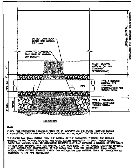
CITY OF RAPID CITY PUBLIC WORKS DEPARTMENT TYPICAL TRENCH CHECK DAM DETAIL FOR WATER & SEWER MAINS DATE 5-1-07 SEC SHT 11-2
