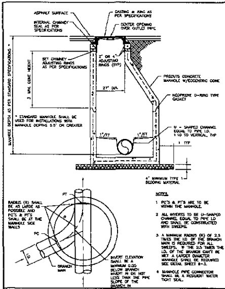
CITY OF RAPID CITY PUBLIC WORKS DEPARTMENT STANDARD MANHOLE DETAIL WITH MONOLITHIC BASE (48" & 60") DATE 5-1-07 SEC SHT 9-1
