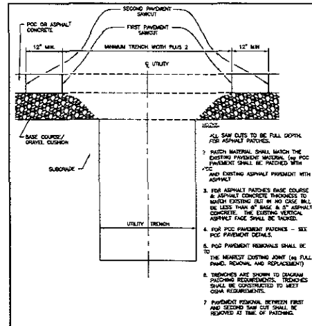
CITY OF RAPID CITY PUBLIC WORKS DEPARTMENT UTILITY TRENCH PATCH DETAIL DATE 5-1-07 SEC SHT 41-1
