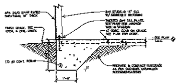
1 SECTION S2 3/4" = 1'-0"
