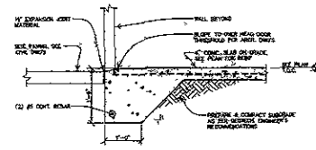
2 SECTION S2 3/4" = 1'-0"
