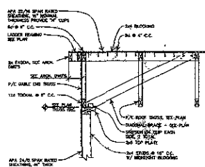
5 SECTION S2 3/4" = 1'-0"
