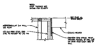
7 SECTION S2 3/4" = 1'-0"
