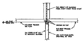
8 SECTION S2 3/4" = 1'-0"
