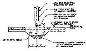
3 SECTION S2 3/4" = 1'-0"
