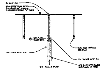
6 SECTION S2 3/4" = 1'-0"
