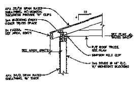
4 SECTION S2 3/4" = 1'-0"
