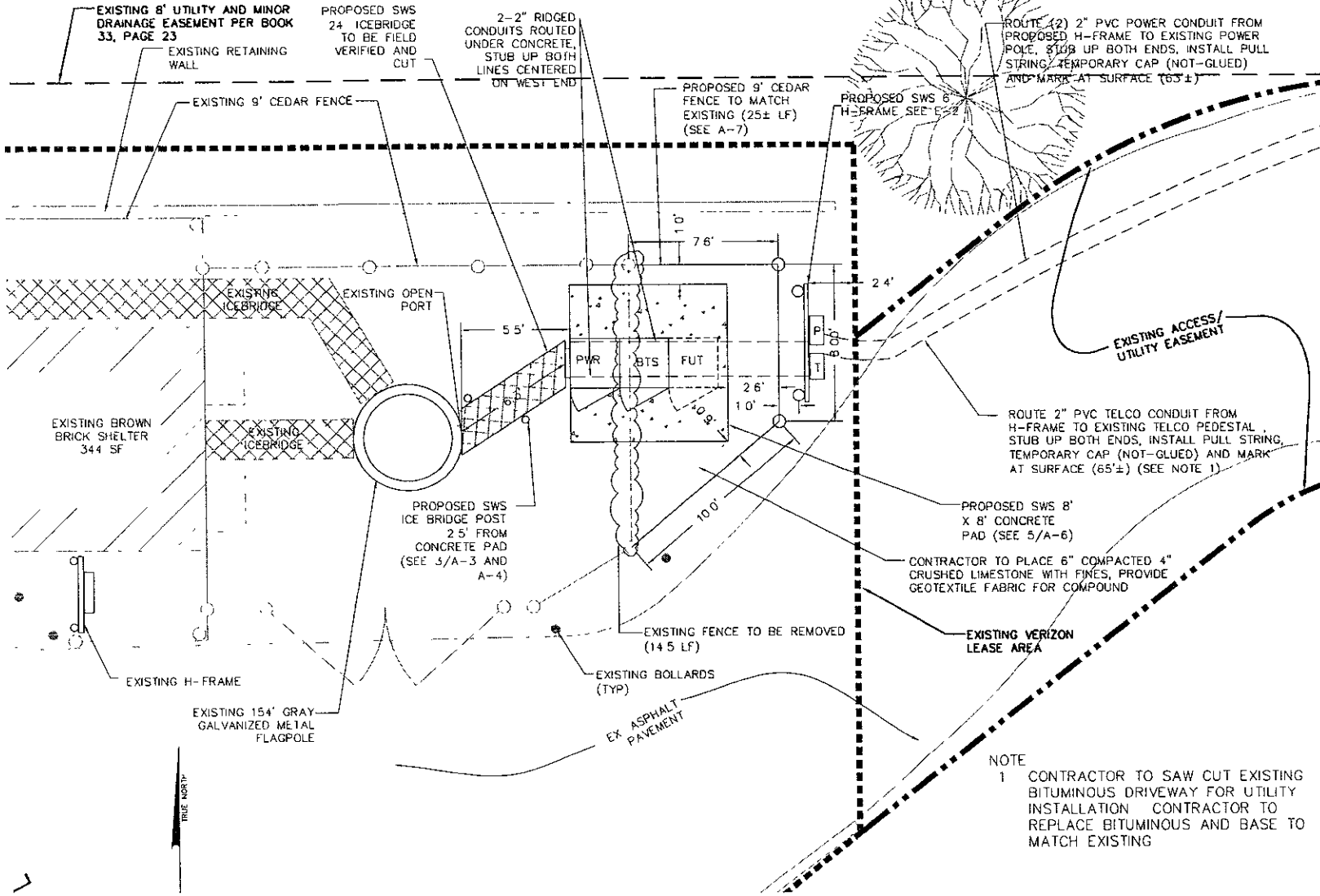
1 COMPOUND PLAN
