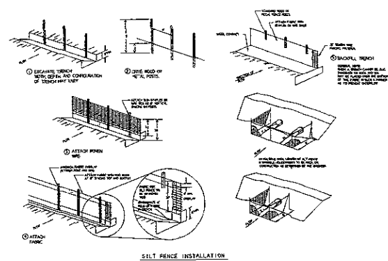
SILT FENCE INSTALLATION
