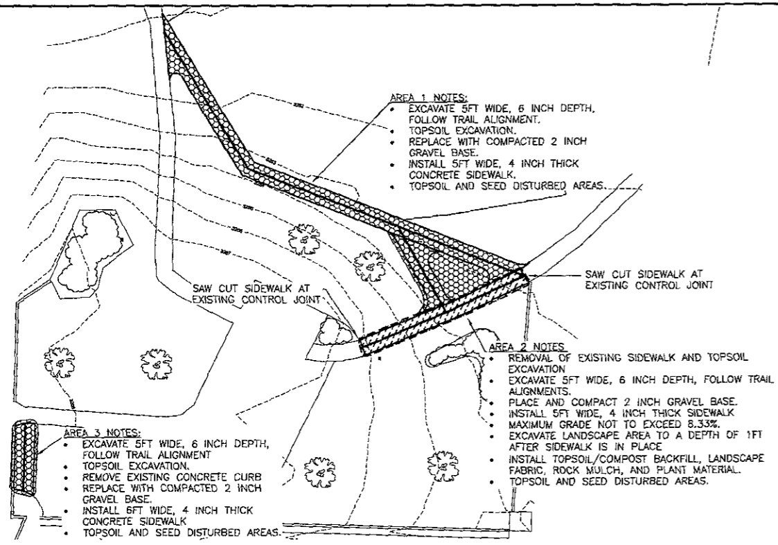
DEMOLITION PLAN SCALE = 1" = 20'
