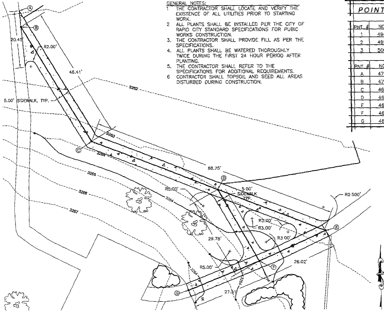
LAYOUT PLAN SCALE = 1" = 10'
