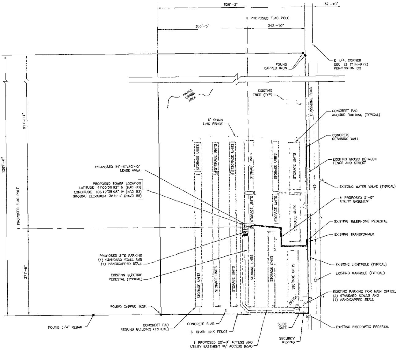
1 OVERALL SITE PLAN SCALE 1"=80'-0"
