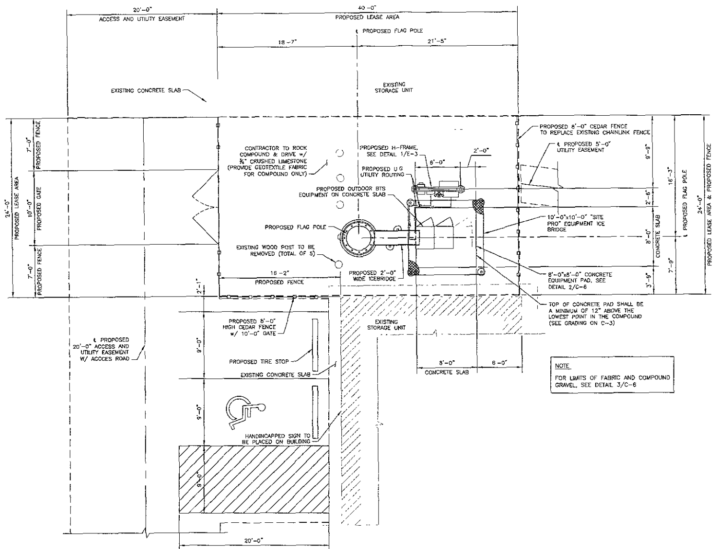
1 COMPOUND PLAN SCALE 1/4"=1'-0"
