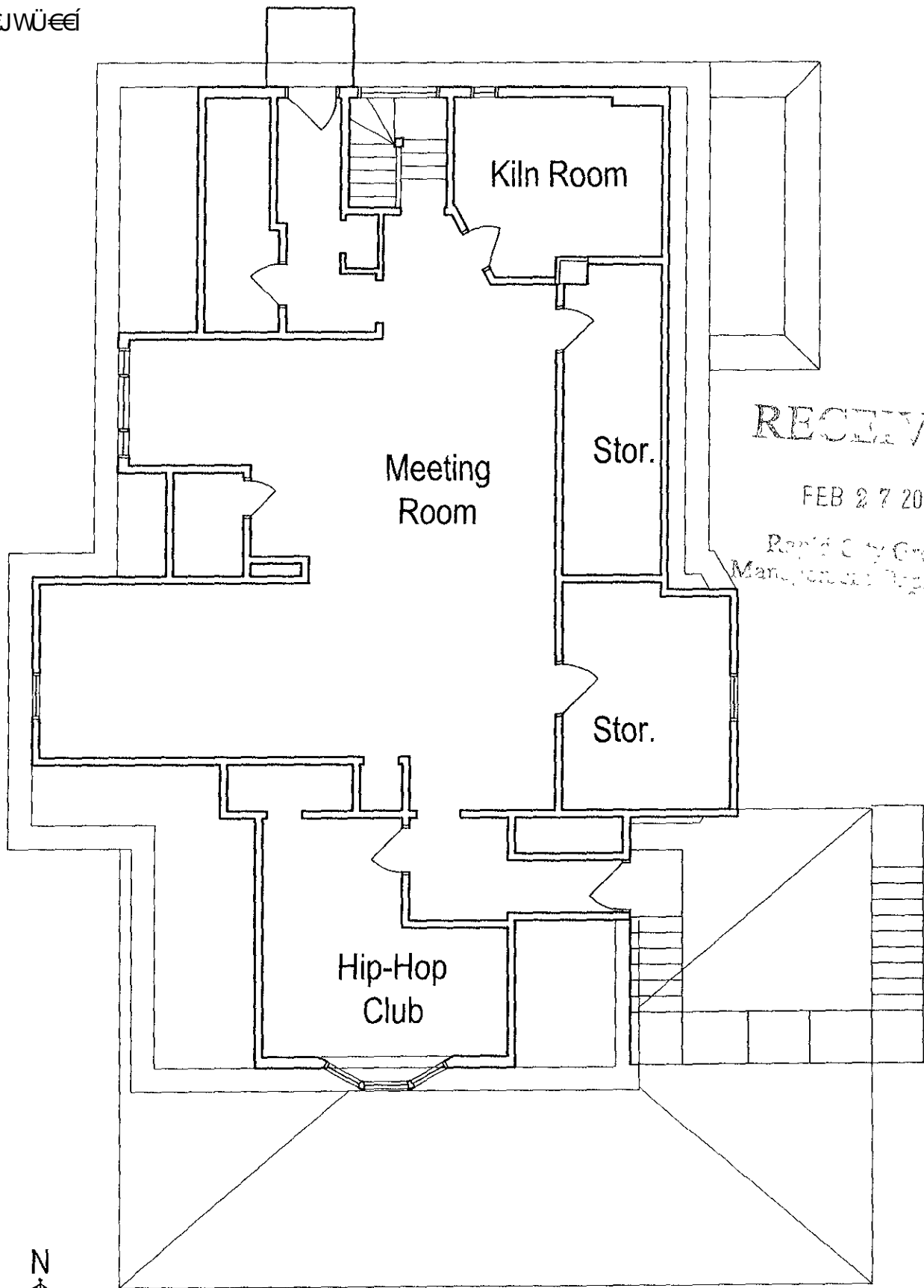
Third Floor Plan @ 1/8" = 1'-0"
