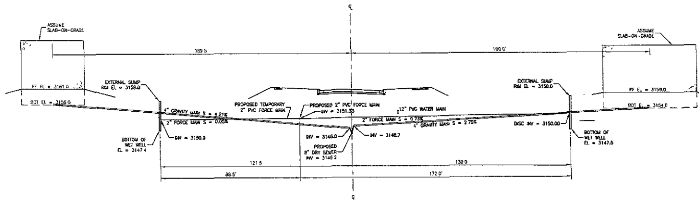
TYPICAL FORCE MAIN SERVICE CROSS SECTION
