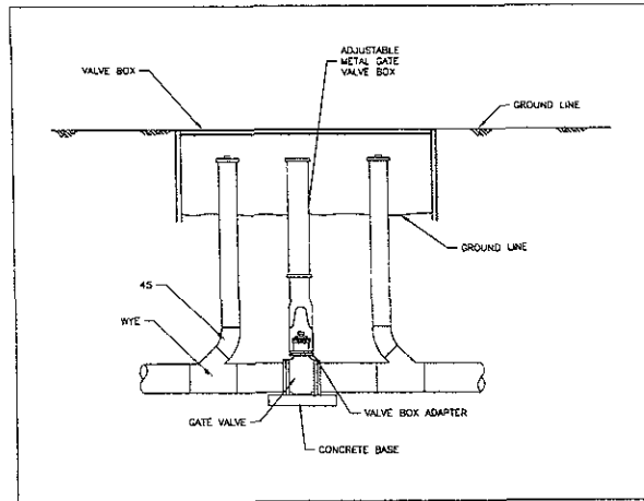
FORCE MAIN CLEANOUT
