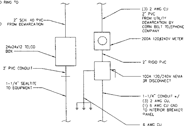
2 UTILITY ONE LINE SCALE NONE
