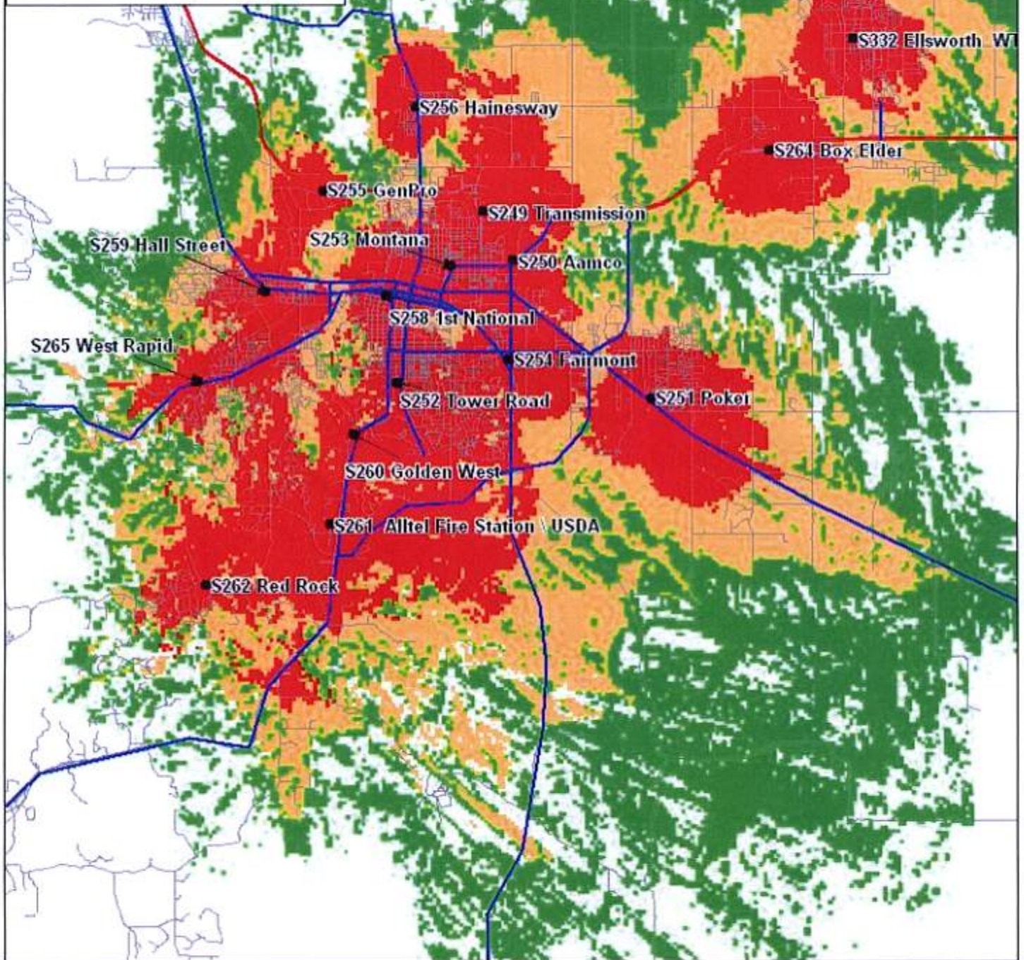
This RF coverage plot is based on an open rural topographical model. Coverage levels are predicted and are not a guarantee of actual or operational coverage.
