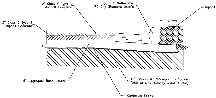
TYPICAL NEW PAVEMENT SECTION NO SCALE
