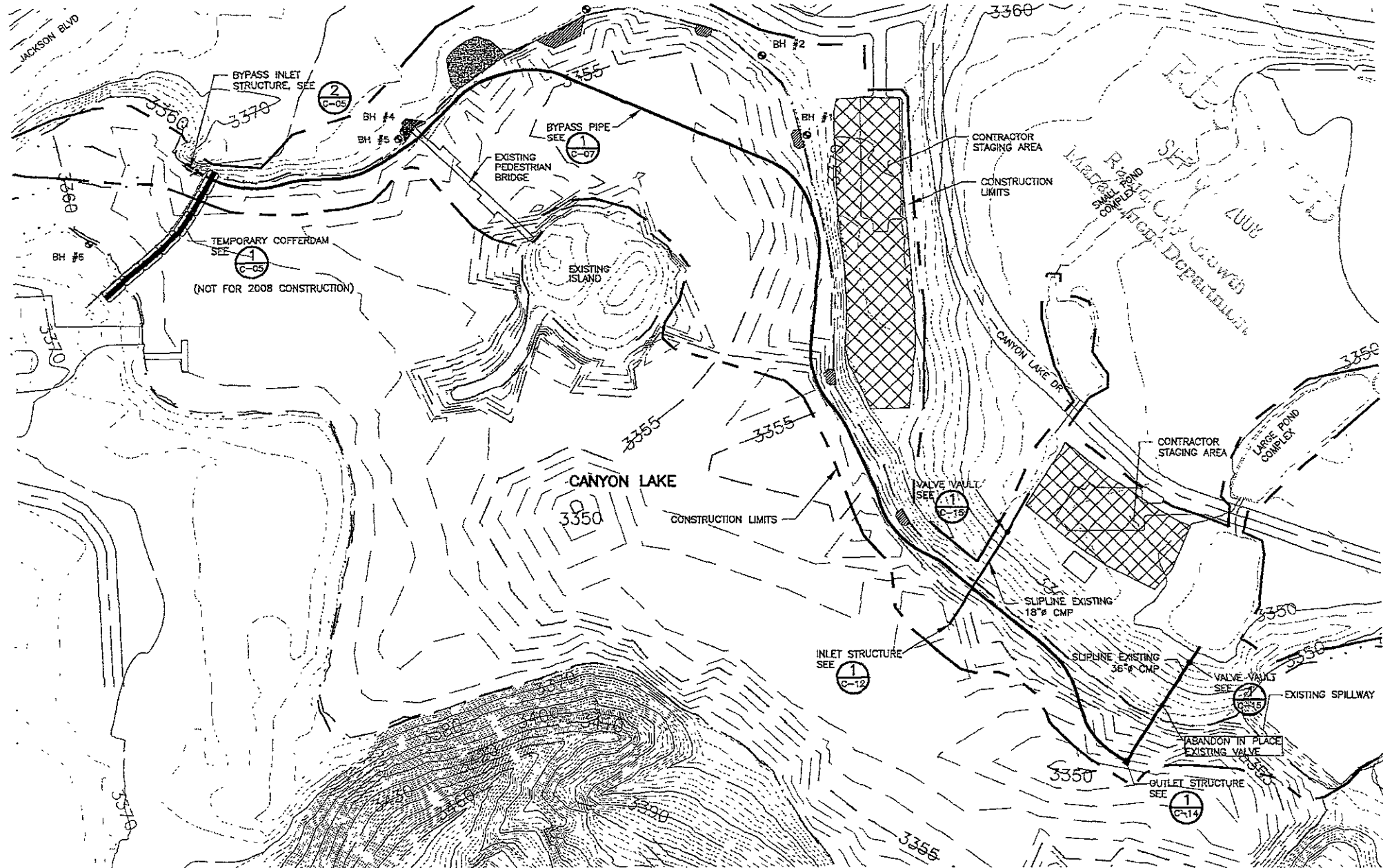
Figure 1-1 PROJECT LAYOUT Canyon Lake Bypass State of South Dakota
