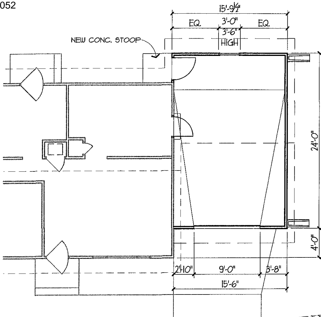
1 A1 FLOOR PLAN 1/8" = 1'-0"
