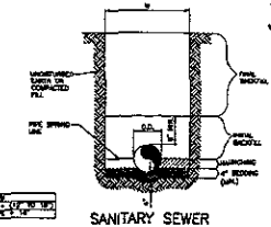
SANITARY SEWER DETAIL NO SCALE
