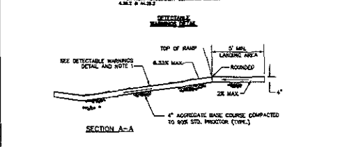
RAMP IN SIDEWALK DETAIL NO SCALE
