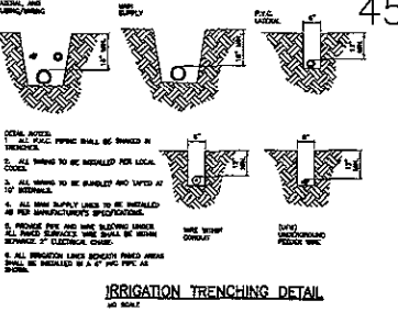
IRRIGATION TRENCHING DETAIL NO SCALE
