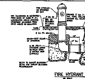
FIRE HYDRANT ASSEMBLY DETAIL NO SCALE
