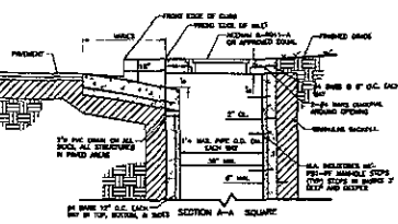
TYPE "A" TOP CATCH BASIN DETAIL NO SCALE
