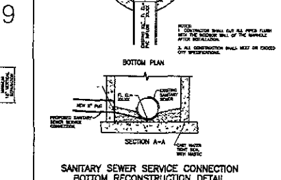
SANITARY SEWER SERVICE CONNECTION BOTTOM RECONSTRUCTION DETAIL NO SCALE
