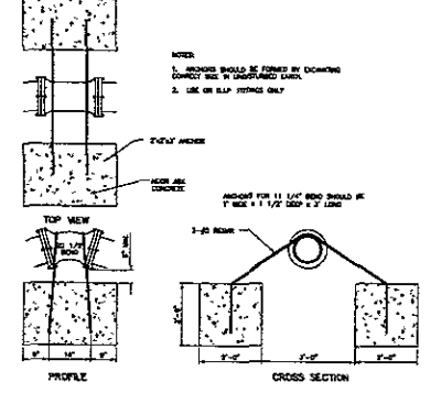
WATER LINE ANCHORING DETAIL NO SCALE
