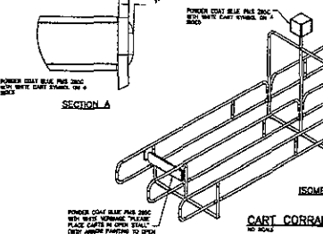
CART CORRAL DETAIL NO SCALE
