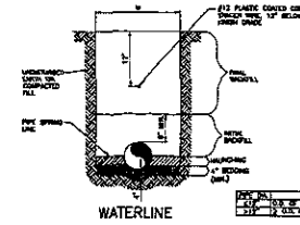
WATERLINE DETAIL NO SCALE
