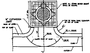
PLAN OF GUTTER SUMP NO SCALE
