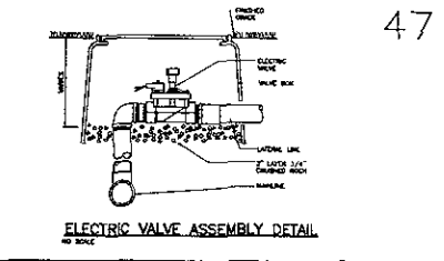
ELECTRIC VALVE ASSEMBLY DETAIL NO SCALE
