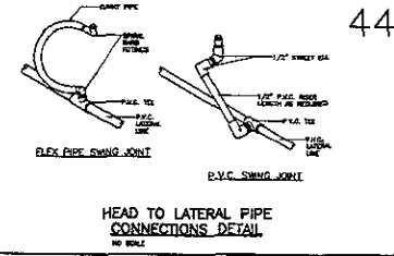
HEAD TO LATERAL PIPE CONNECTIONS DETAIL NO SCALE
