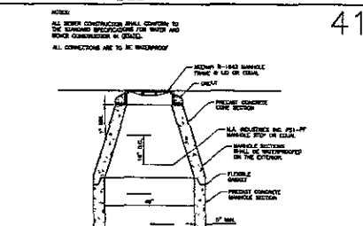
STANDARD SANITARY SEWER MANHOLE DETAIL NO SCALE
