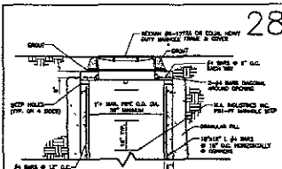
JUNCTION BOX DETAIL NO SCALE
