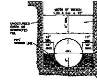
ALL PIPE SIZES AND MATERIAL INCLUDING REINFORCED CONCRETE PIPE 60" S AND LARGER
