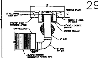
STORM SEWER CLEANOUT DETAIL NO SCALE
