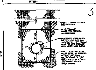
DRAIN TILE DETAIL NO SCALE
