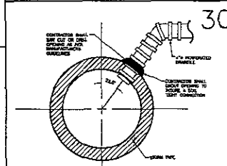
STORM SEWER CLEANOUT DETAIL NO SCALE
