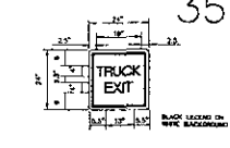
"TRUCK EXIT" SIGN NO SCALE
