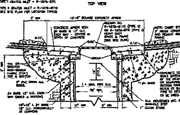
GRADED INLET DETAIL NO SCALE
