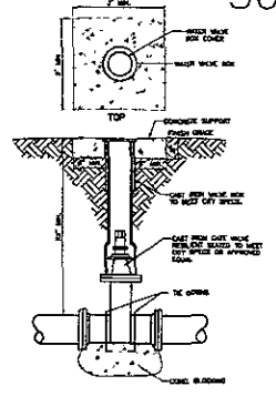
GATE VALVE & VALVE BOX DETAIL NO SCALE
