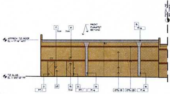
3 SOUTH ELEVATION + . . . 2
