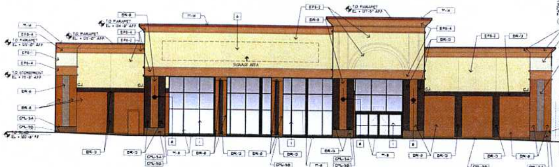
1 NORTH ELEVATION A - C
