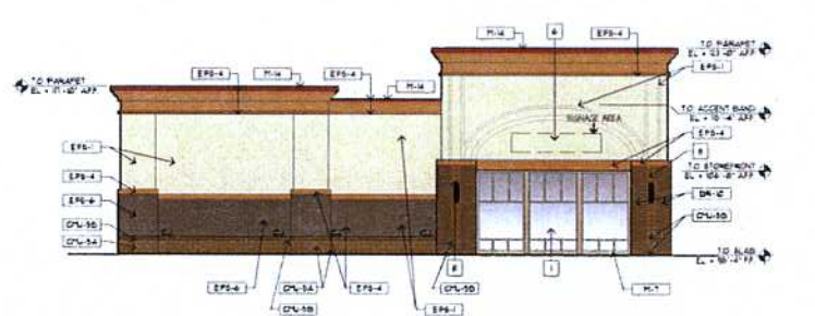
2 EAST ELEVATION 4'-11/2"
