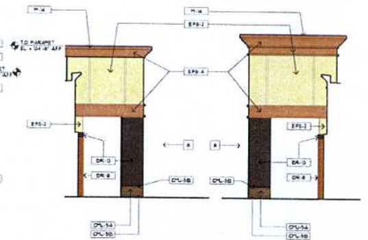
2 EAST ELEVATION AT CANOPY A - C
