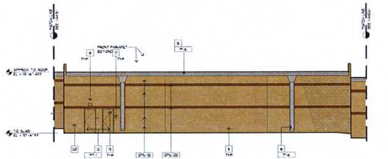
2 SOUTH ELEVATION
