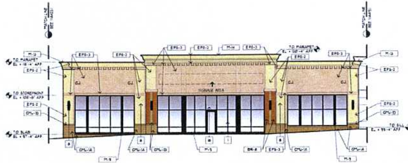
1 NORTH ELEVATION
