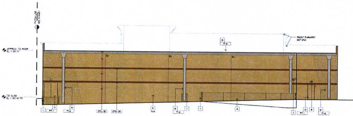
4 SOUTH ELEVATION A - C
