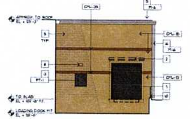
5 WEST ELEVATION (LOADING DOCK) A - C
