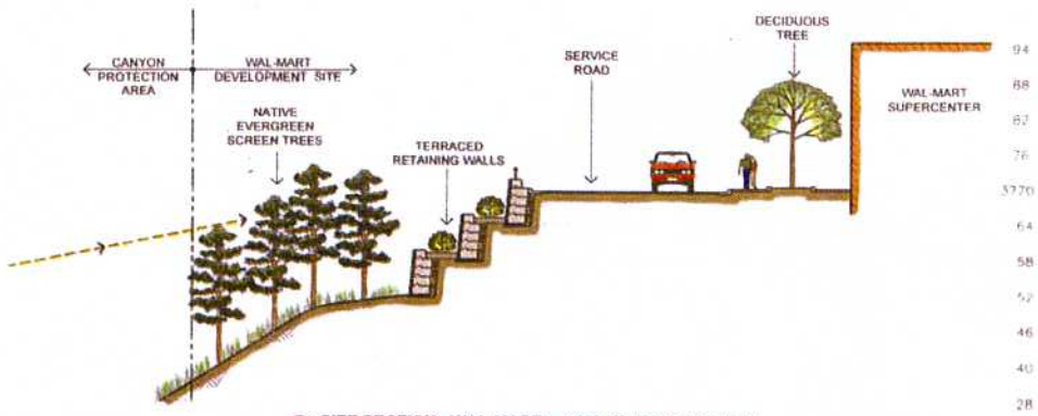
B SITE SECTION: WAL-MART ←→ NORTHEAST CANYON SCALE: 3/32"=1'-0"
