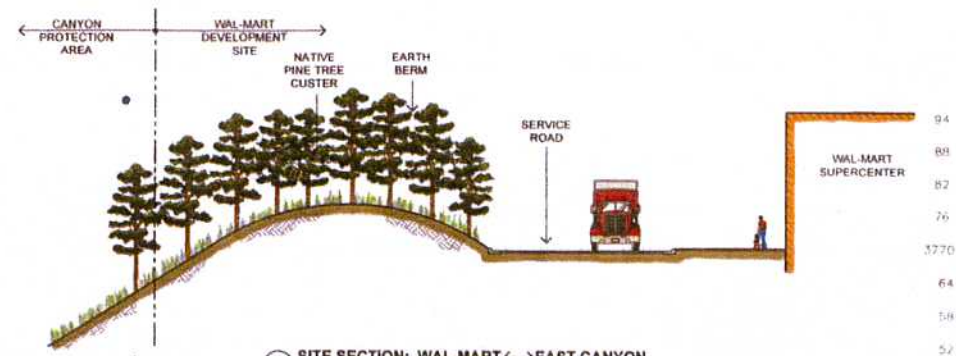
A SITE SECTION: WAL-MART ←→ EAST CANYON SCALE: 3/32"=1'-0"
