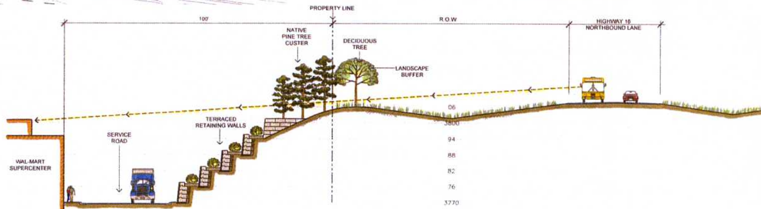
C SITE SECTION: WAL-MART ←→ EAST CANYON SCALE: 3/32"=1'-0"
