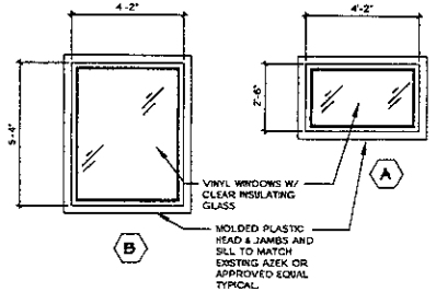
WINDOW ELEVATION SCALE 1/2" = 1'-0"
