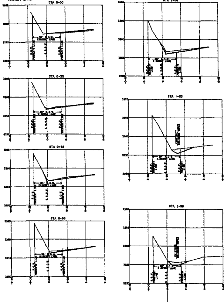
6 CROSS-SECTIONS KIRKEY LANE
