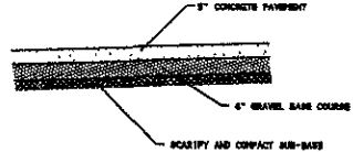
PAVEMENT SECTION KIRKEY LANE
