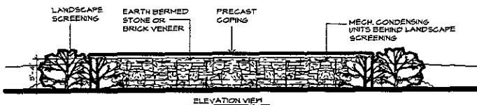
DUMPSTER ENCLOSURE SCALE 1/4" = 1'-0"
