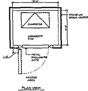
DUMPSTER ENCLOSURE SCALE 1/4" = 1'-0"
