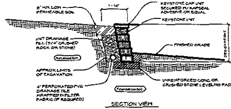
RETAINING WALL DETAIL SCALE 1/2" = 1'-0"
