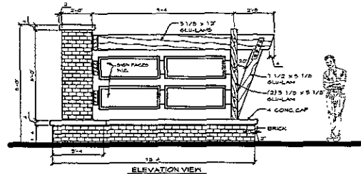
BUILDING IDENTIFICATION SIGN 'B' SCALE 3/8" = 1'-0"
