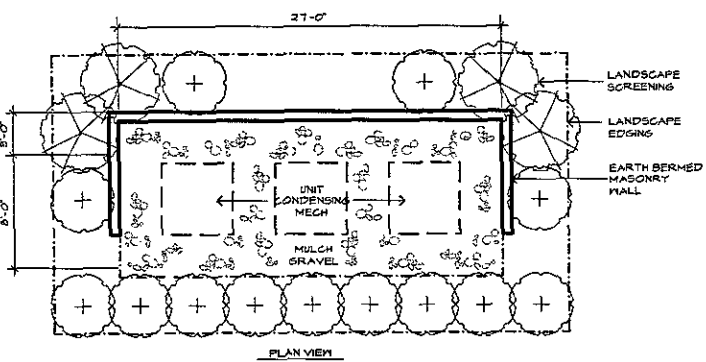
MECHANICAL ENCLOSURE SCALE 1/4" = 1'-0"
