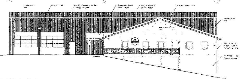
B1 EXTERIOR ELEVATIONS
