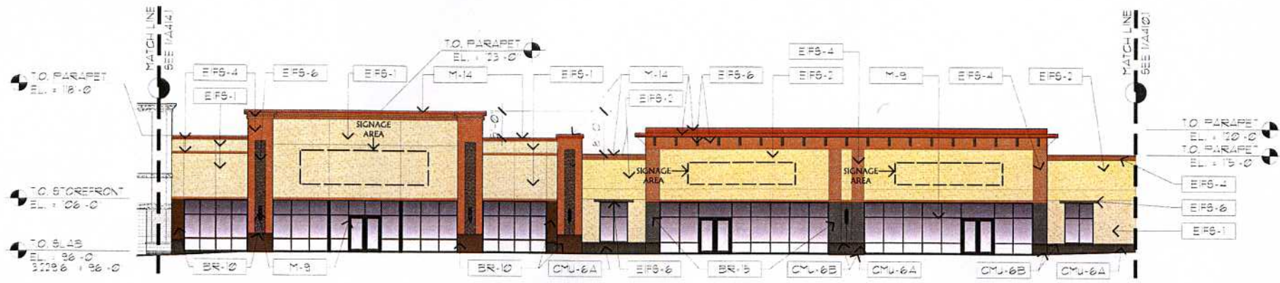
1 NORTH ELEVATION 1/8" = 1'-0"
