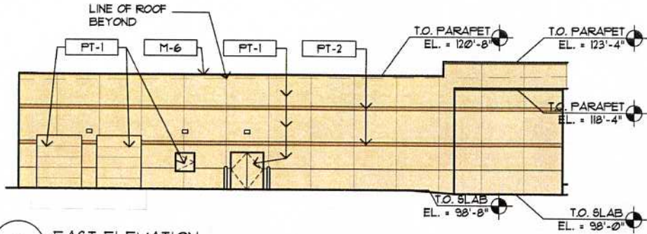
3 EAST ELEVATION 1/16" = 1'-0"
