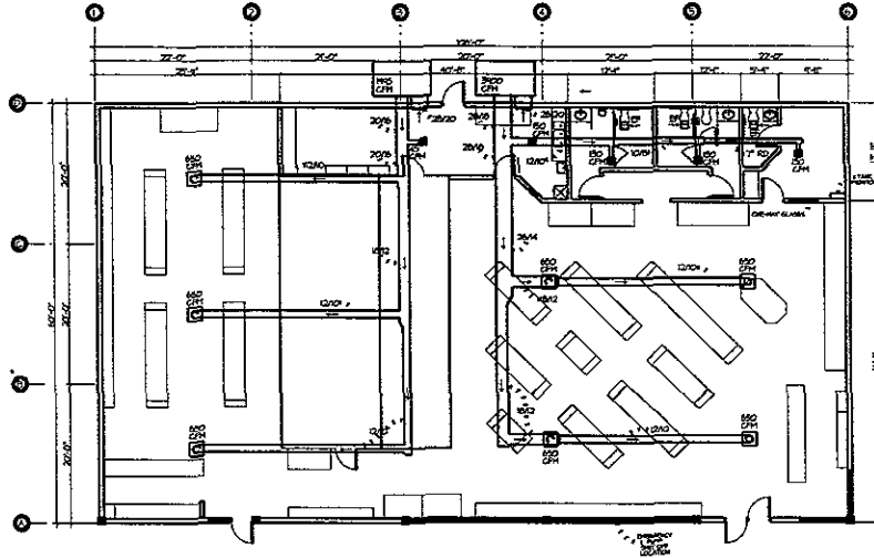
HVAC PLAN
