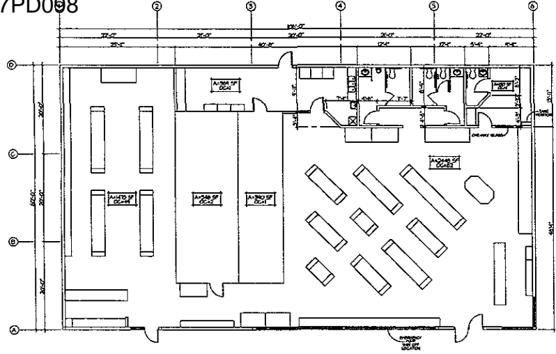
FLOOR PLAN
