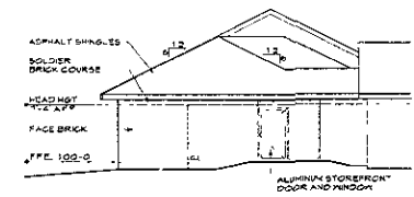
6 SOUTHEAST ELEVATION 0511S (REV. 05)
