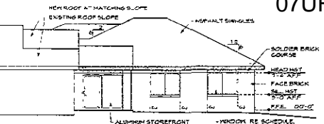
1 NORTH ELEVATION 0511S (REV. 05)
