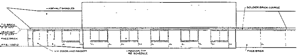
4 SOUTHWEST ELEVATION #1 0511S (REV. 05)
