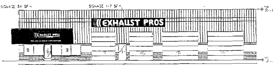
East Elevation SCALE 1/16" = 1'-0"
