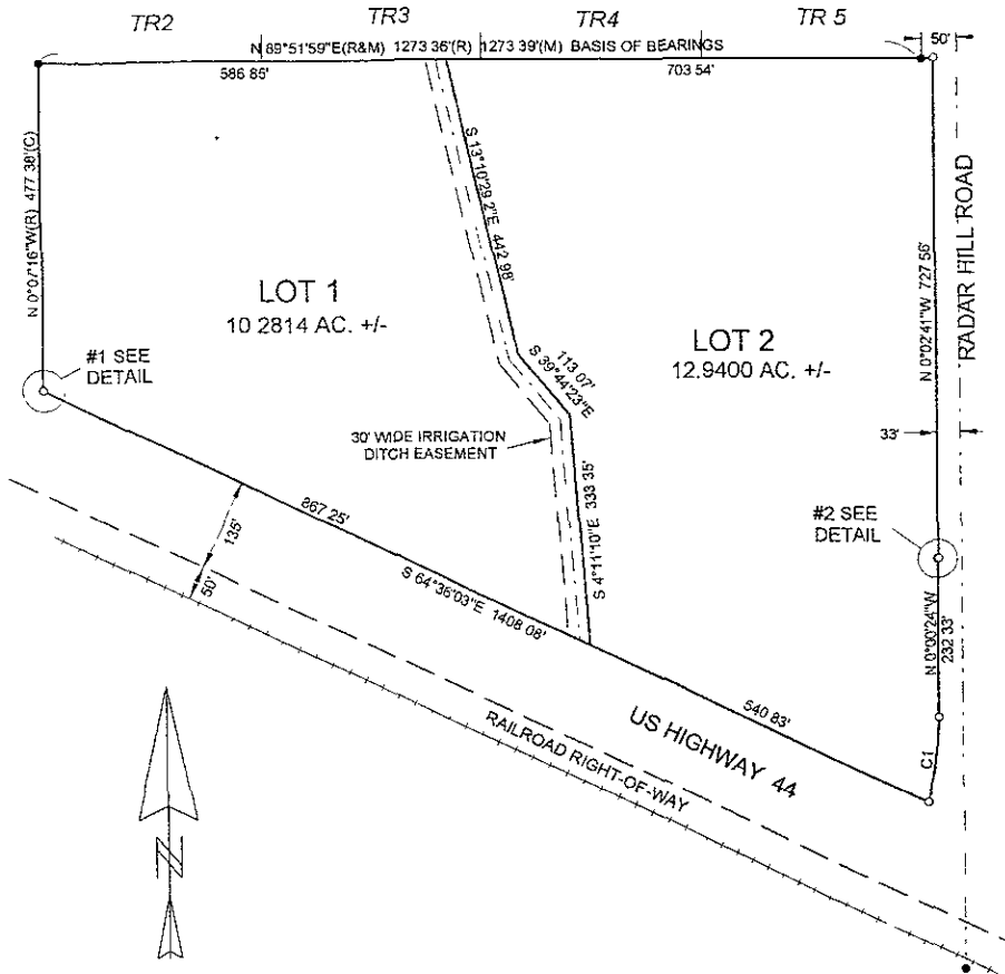
LAYOUT PLAT OF LOTS 1 & 2 OF POWDERHORN SUBDIVISION (FORMERLY UNPLATTED SE1/4NE1/4 NORTH OF HWY 44 AND LESS HIGHWAY LOTS) LOCATED IN SE1/4NE1/4 OF SECTION 24, T1N, R8E, B H M. PENNINGTON COUNTY, SOUTH DAKOTA
