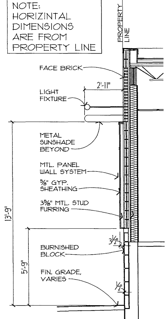
1 WALL SECTION 1/4" = 1'-0"
