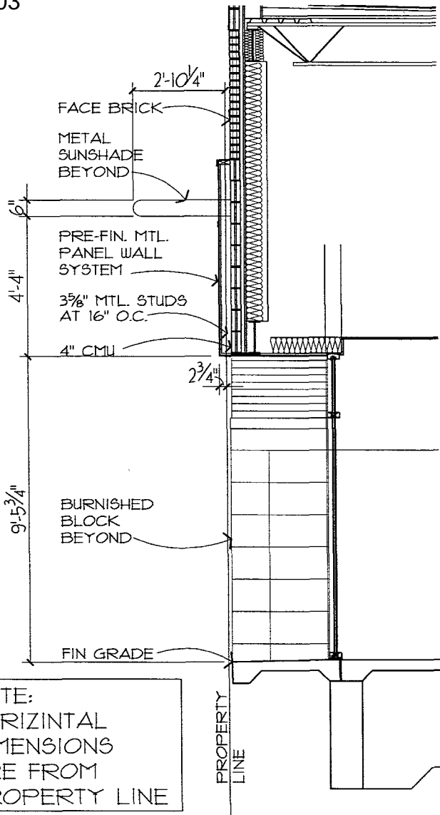
1 WALL SECTION 1/4" = 1'-0"
