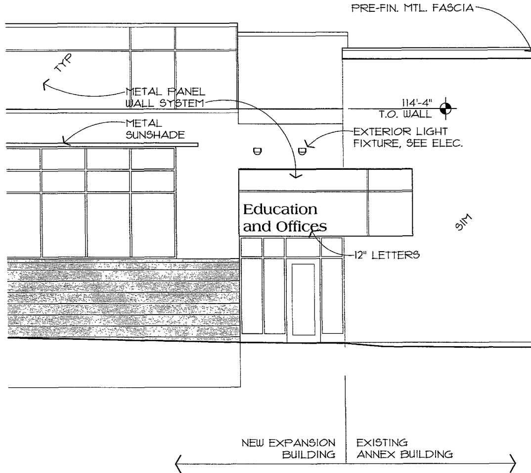
2 PARTIAL EAST ELEVATION 1/8" = 1'-0"
