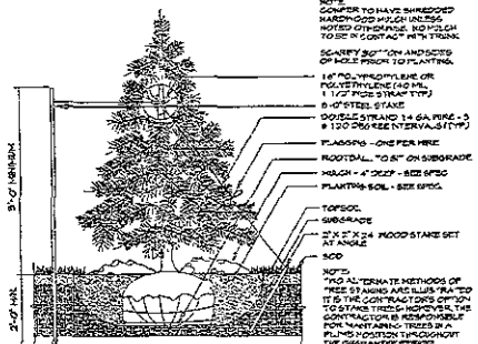
1 CONIFEROUS TREE IN MULCH N.T.S.
