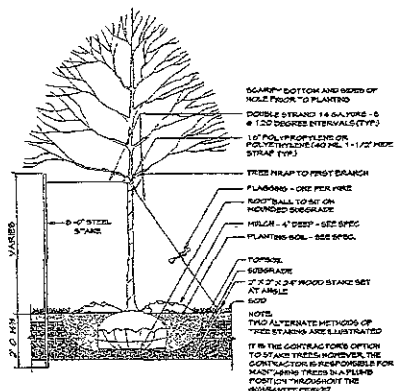
2 DECIDUOUS TREE IN MULCH N.T.S.
