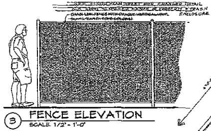
3 FENCE ELEVATION SCALE 1/2\"/>
