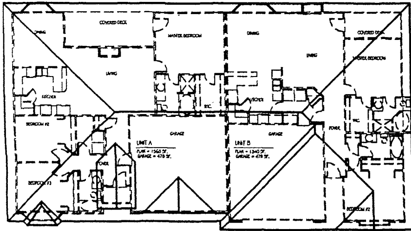
ROOF PLAN
