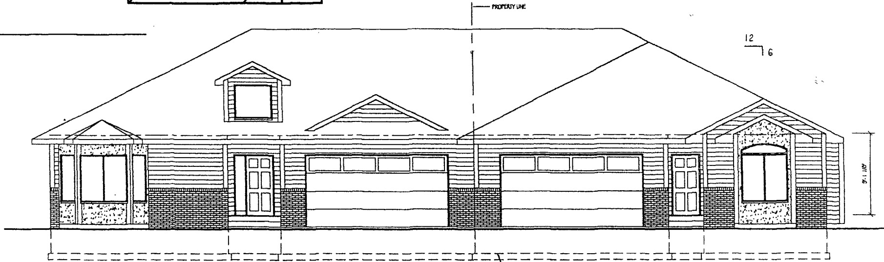
FRONT ELEVATION
