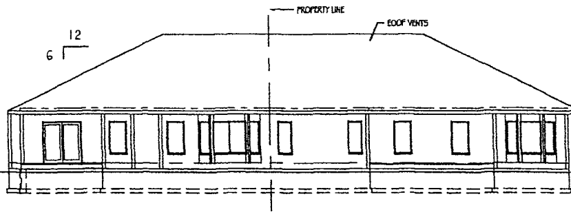
REAR ELEVATION
