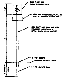
HANDICAP SIGN NOT TO SCALE
