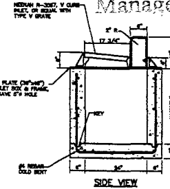
TYPE "B" INLET (MODIFIED) NOT TO SCALE
