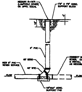
SEWER CLEANOUT DETAIL NOT TO SCALE
