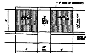
HANDICAP RAMP NOT TO SCALE
