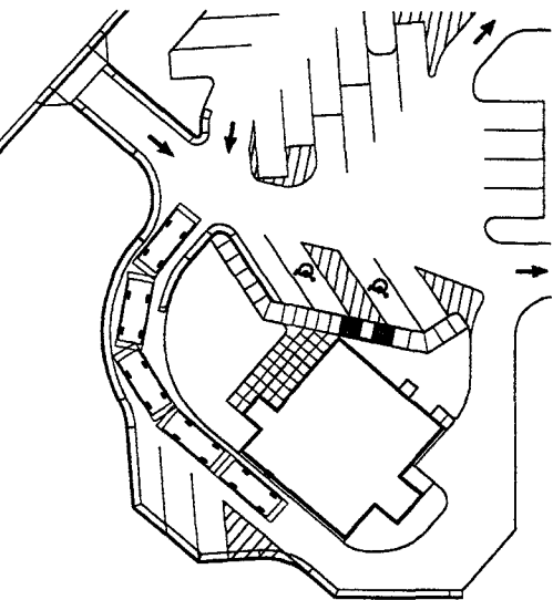
DRIVE THRU STACKING SCALE: 1"=20'
