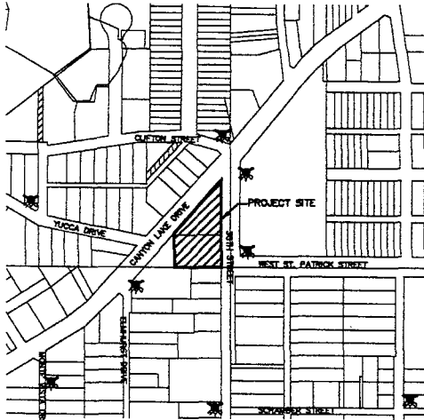
FIRE HYDRANT LOCATION MAP SCALE: 1"=200'
