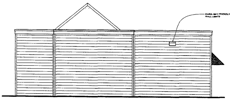
3 EAST ELEVATION SCALE: 1/4" = 1'-0"
