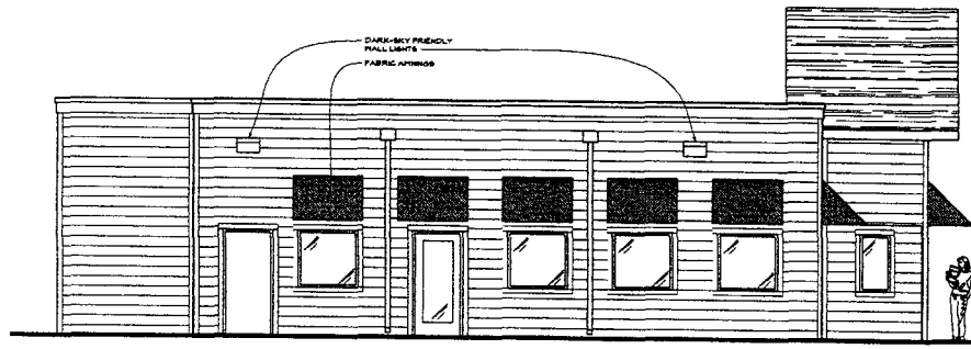
4 NORTH ELEVATION SCALE: 1/4" = 1'-0"
