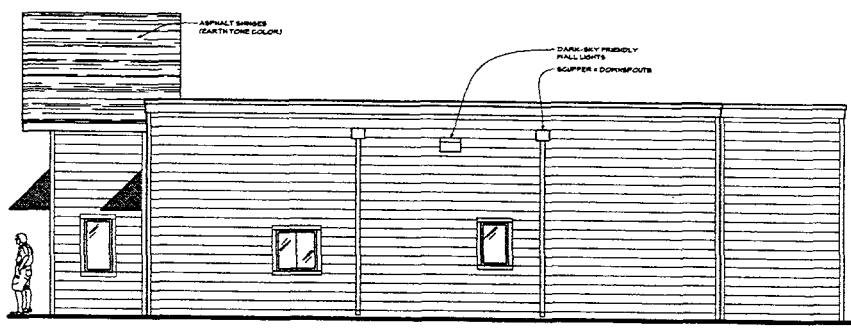
2 SOUTH ELEVATION SCALE: 1/4" = 1'-0"
