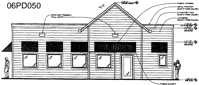
1 WEST ELEVATION SCALE: 1/4" = 1'-0"
