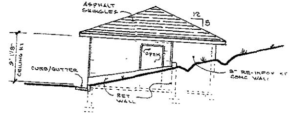
RIGHT (WEST) ELEVATION
