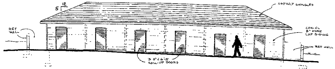
FRONT (NORTH) ELEVATION
