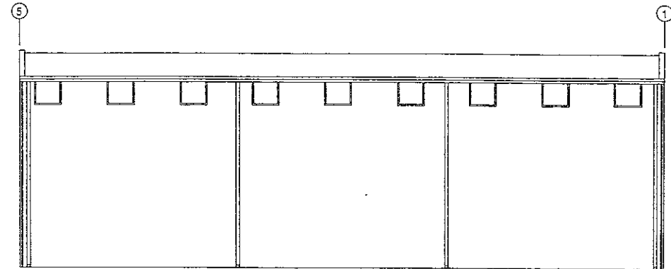
GRID G ELEVATION
