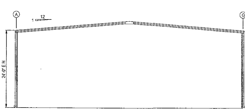
GRID 5 ELEVATION
