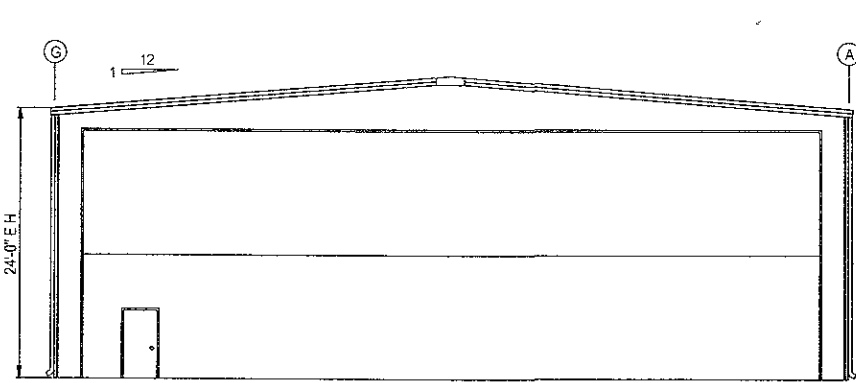
GRID 1 ELEVATION
