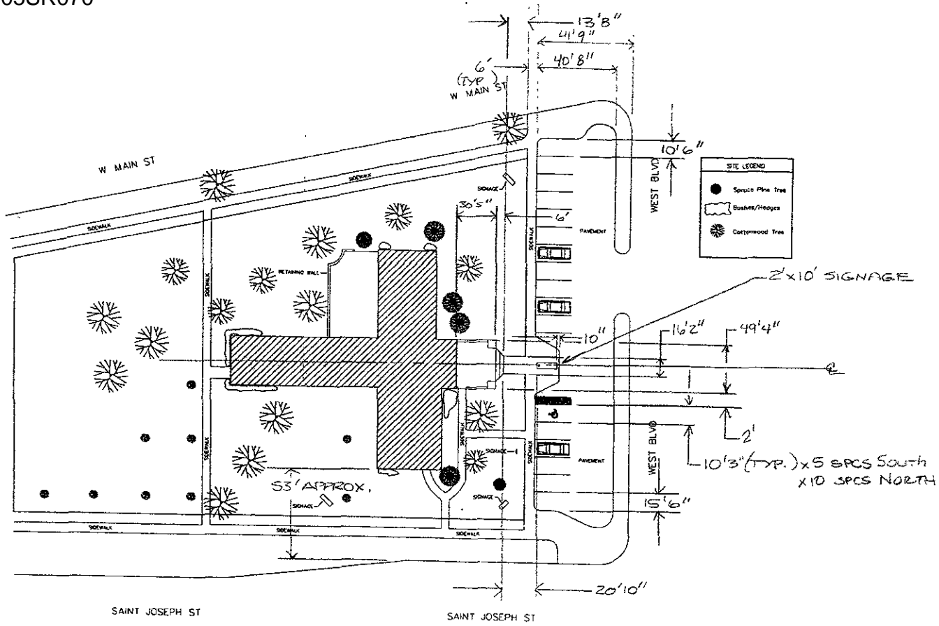
1 SITE PLAN SCALE 1" = 20'-0"
