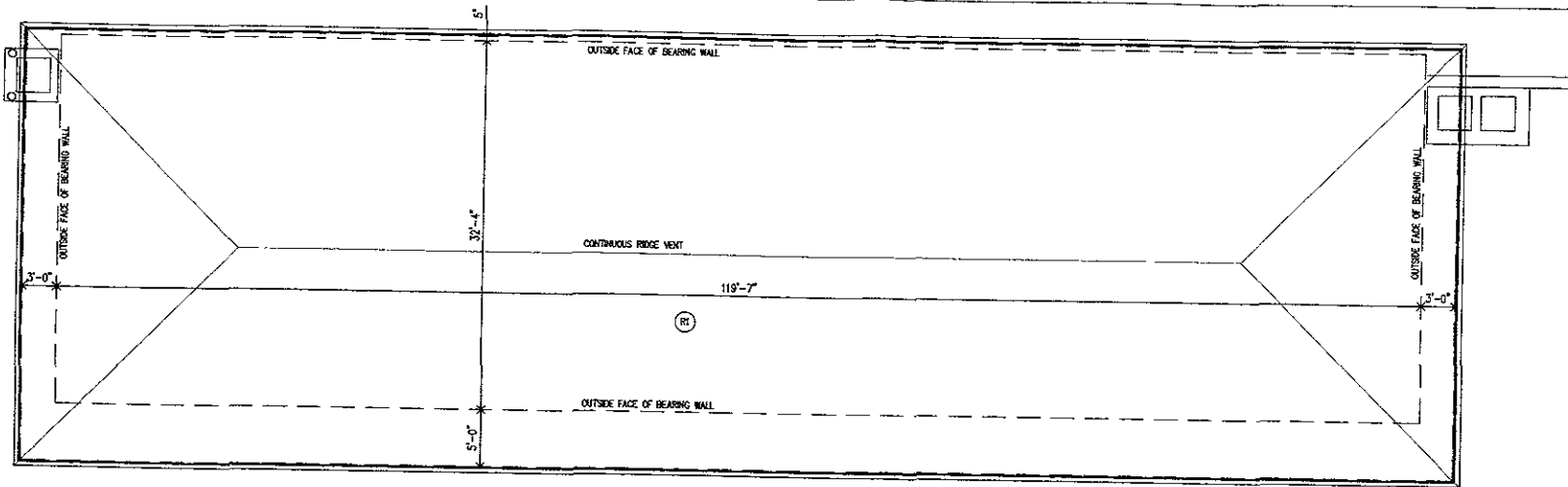
ROOF PLAN SCALE: 3/32" = 1'-0" NORTH
