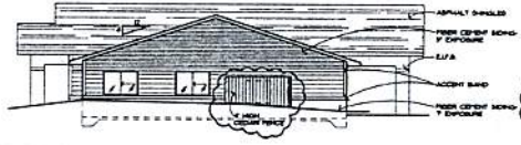
WEST ELEVATION: BUILDING 1
