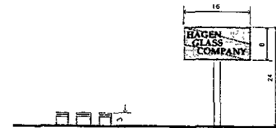
SIGN ELEVATION SCALE UP - 1/4"
