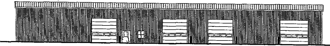
WEST ELEVATION SCALE UP - 1/4"
