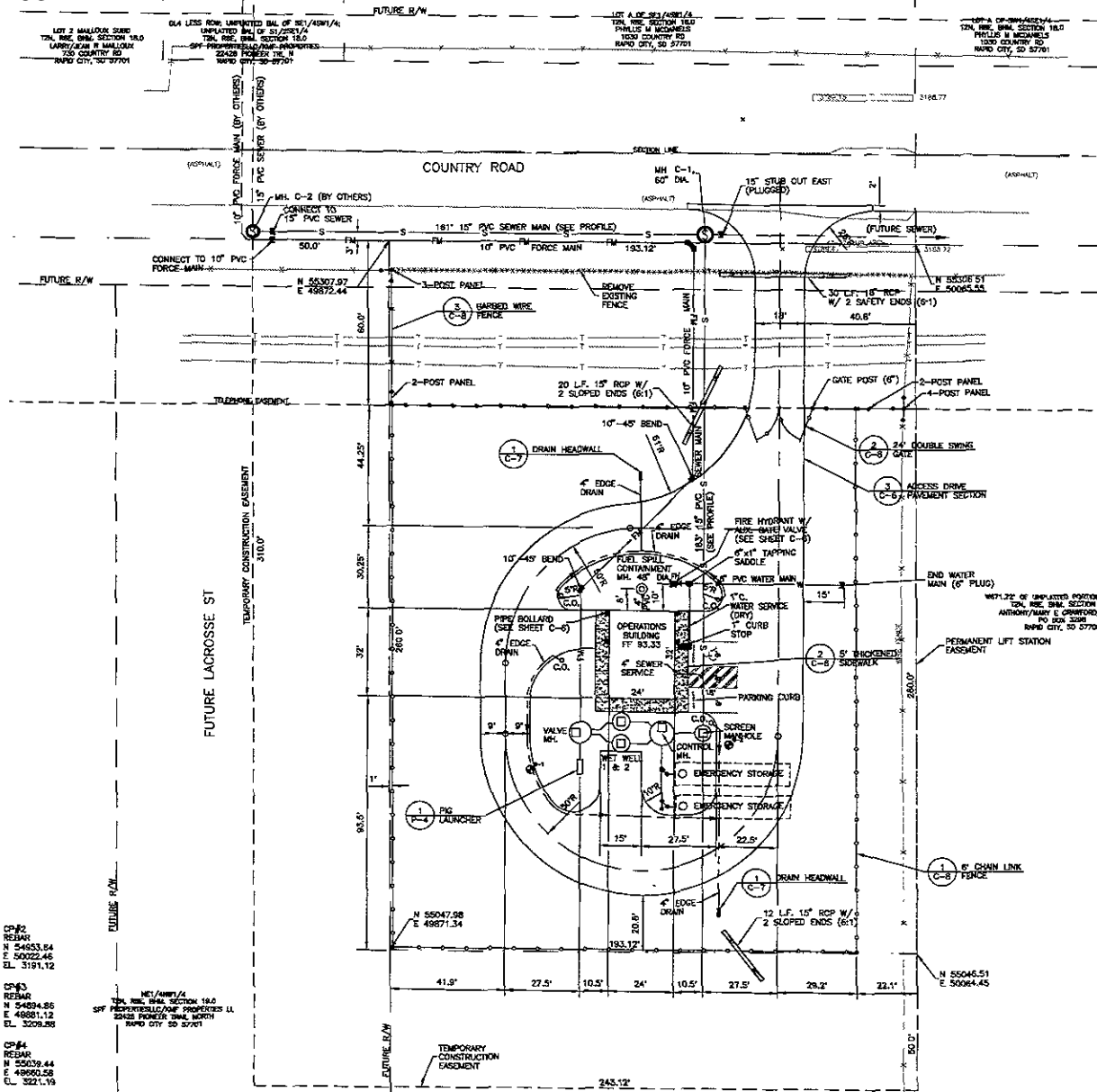
SITE DEVELOPMENT PLAN
