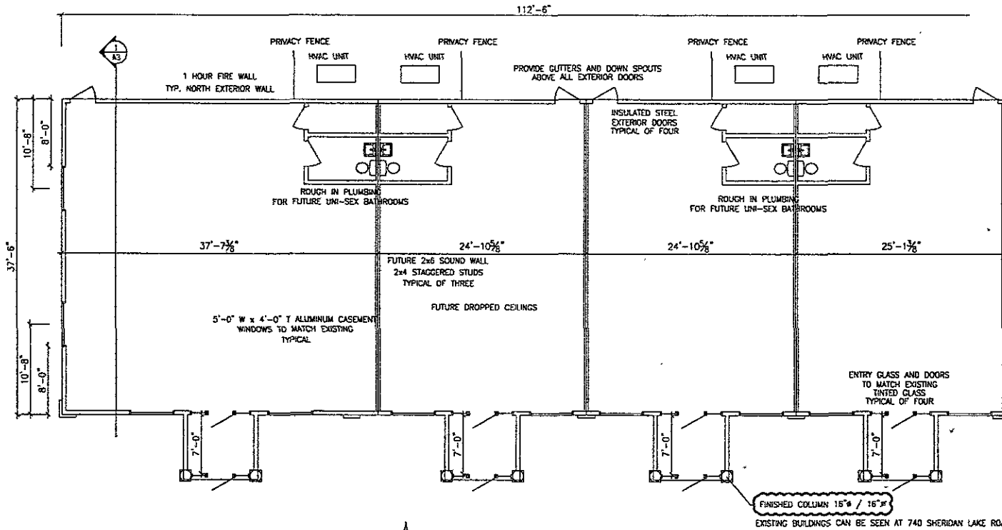
FLOOR PLAN Scale: 3/32" = 1'-0"
