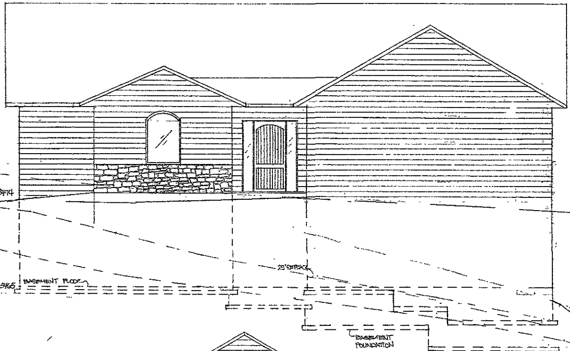
SOUTH (FRONT) ELEVATION 1/4" = 1'-0"
