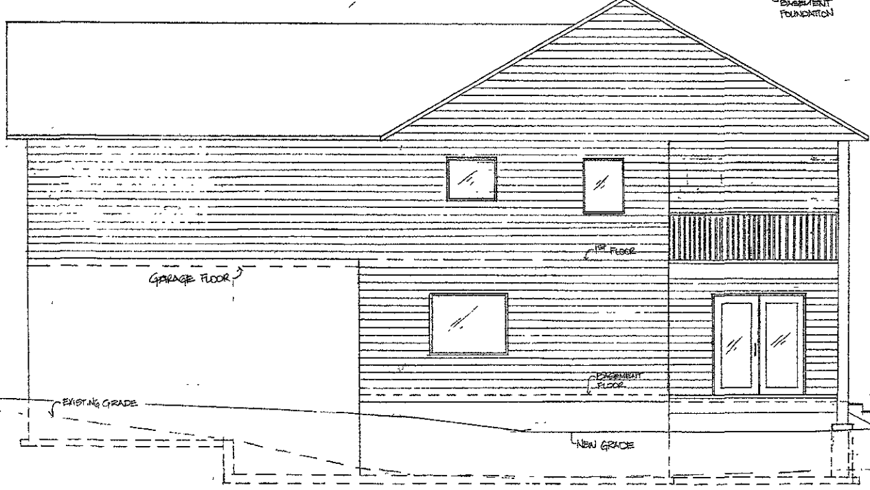
SOUTH (FRONT) ELEVATION 1/4" = 1'-0"
