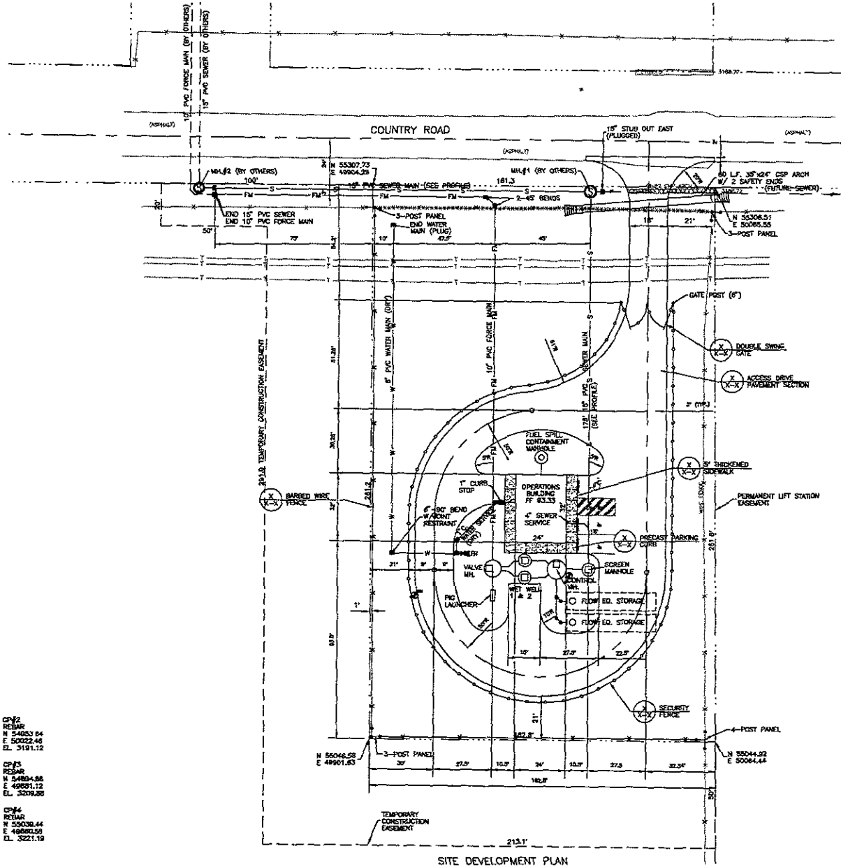
SITE DEVELOPMENT PLAN
